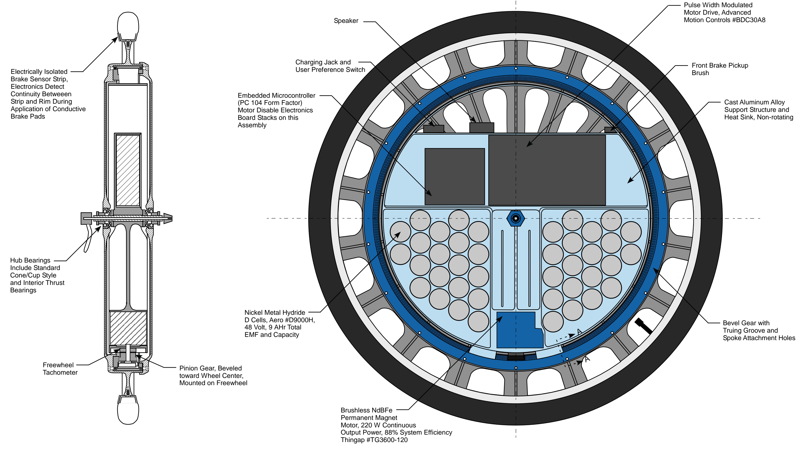
Section with Right Spokes and Bearings in Place
